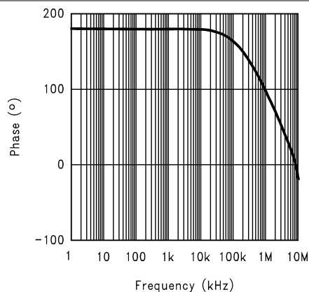
Figure 5-14. Error Amplifier Phase
