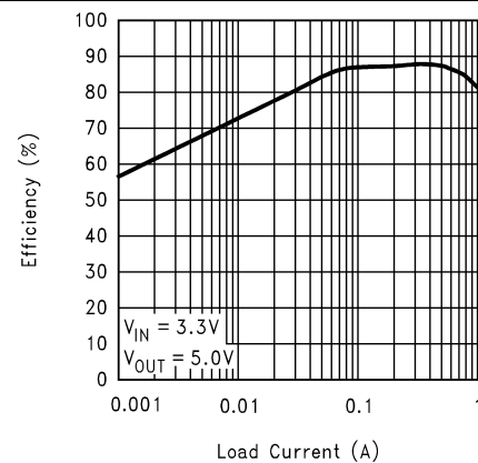
Figure 5-12. Efficiency vs Load Current (3.3V In and 5V Out)
