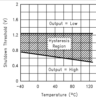
Figure 5-18. Shutdown Threshold Hysteresis vs Temperature
