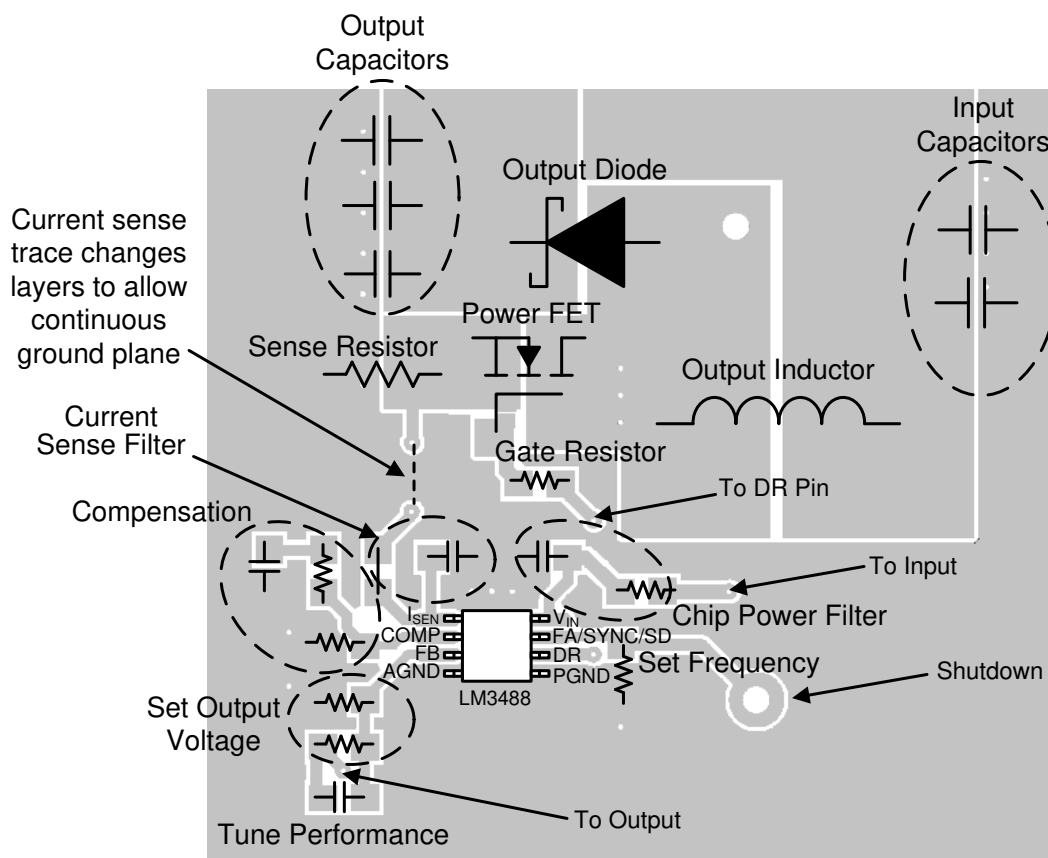
Figure 7-9. Example Layout of a Boost Application using LM3488
