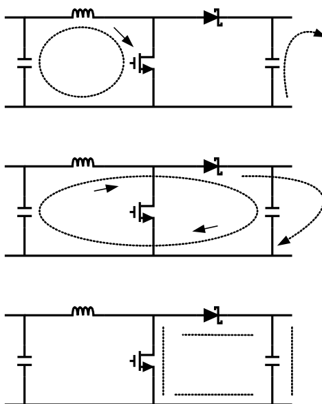
Figure 7-8. Current Flow in a Boost Application
