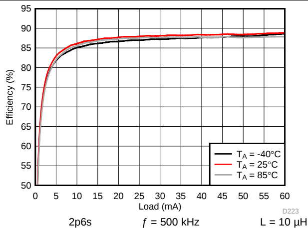
图 91. Backlight Boost Efficiency
