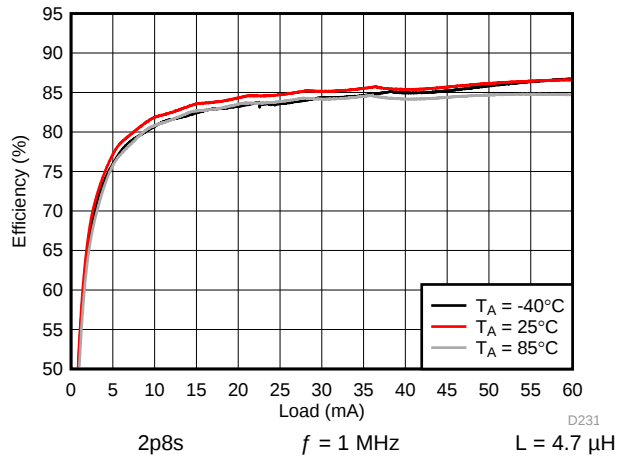
图 99. Backlight Boost Efficiency
