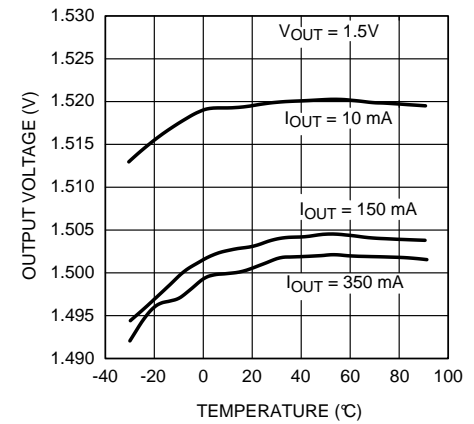
Figure 8. Output Voltage vs. Temperature
