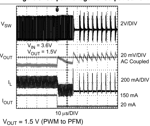
Figure 11. Mode Change by Load Transients
