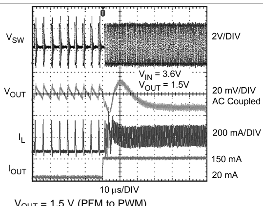
Figure 10. Mode Change by Load Transients
