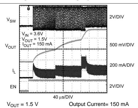
Figure 12. Start-Up into PWM Mode
