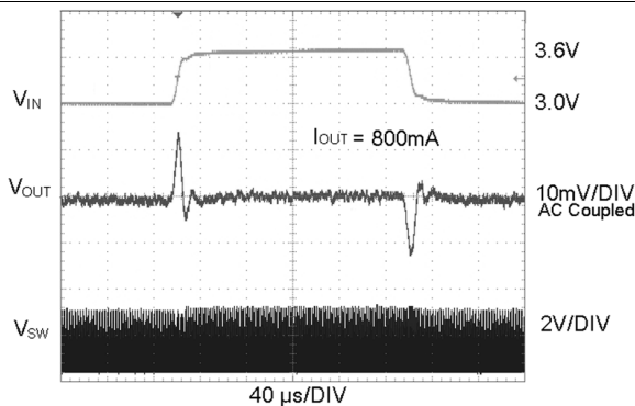
V_{OUT} = 0.75\text{ V}
