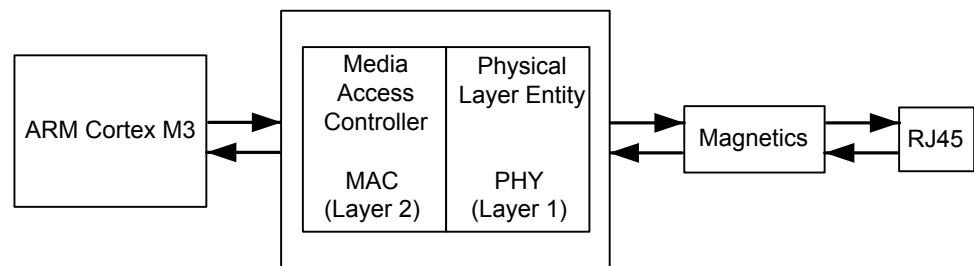
Figure 15-1. Ethernet Controller
