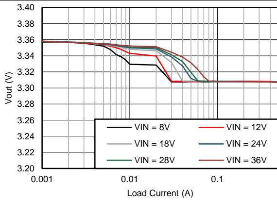
Figure 7. V_{OUT} Regulation
