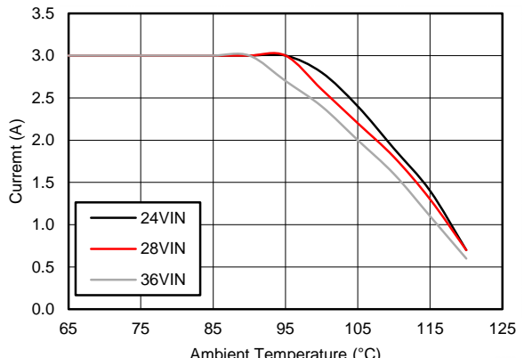
Figure 96. Derating Curve
