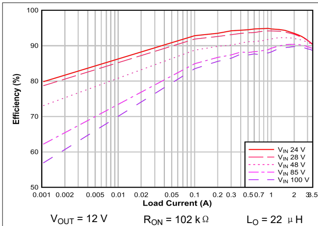
图 8-2. Conversion Efficiency (Log Scale)
