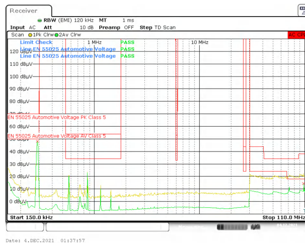
图 8-10. Full-Load Switching
