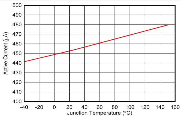
图 6-4. V_{\text{IN}} Active Current Versus Temperature
