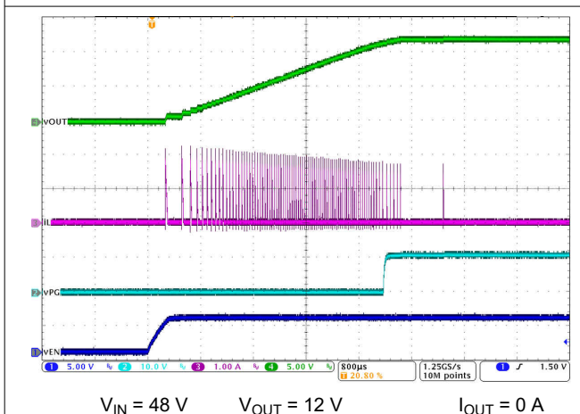
图 8-6. No-Load Start-Up with EN/UVLO
