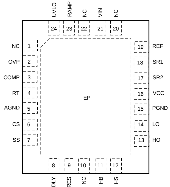
NHZ Package 24-Pin WQFN Top View
