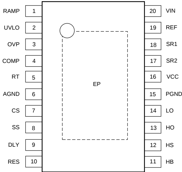
PWP Package 20-Pin HTSSOP With PowerPAD Top View
