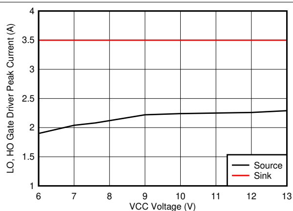
图 7-24. Gate Driver Peak Current vs VCC Voltage
