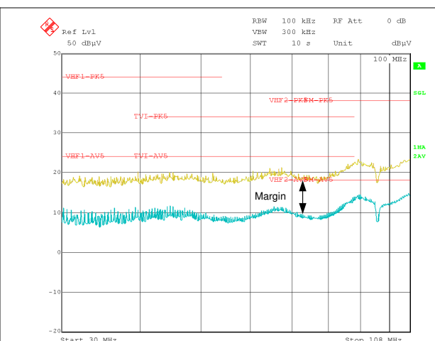
图 9-19. CISPR 25 Class 5 Conducted EMI, 30 MHz to 108 MHz
