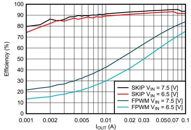
图 10-5. Efficiency vs. I_{OUT} , V_{OUT} = 8.5 -V Light Load
