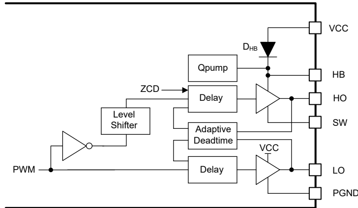
图 9-20. Driver Structure with Internal Boot Diode
