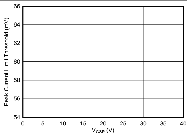
图 8-11. Peak Current Limit Threshold vs V CSP
