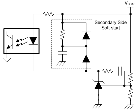
图 8-8. Secondary-Side Soft Start in Flyback
