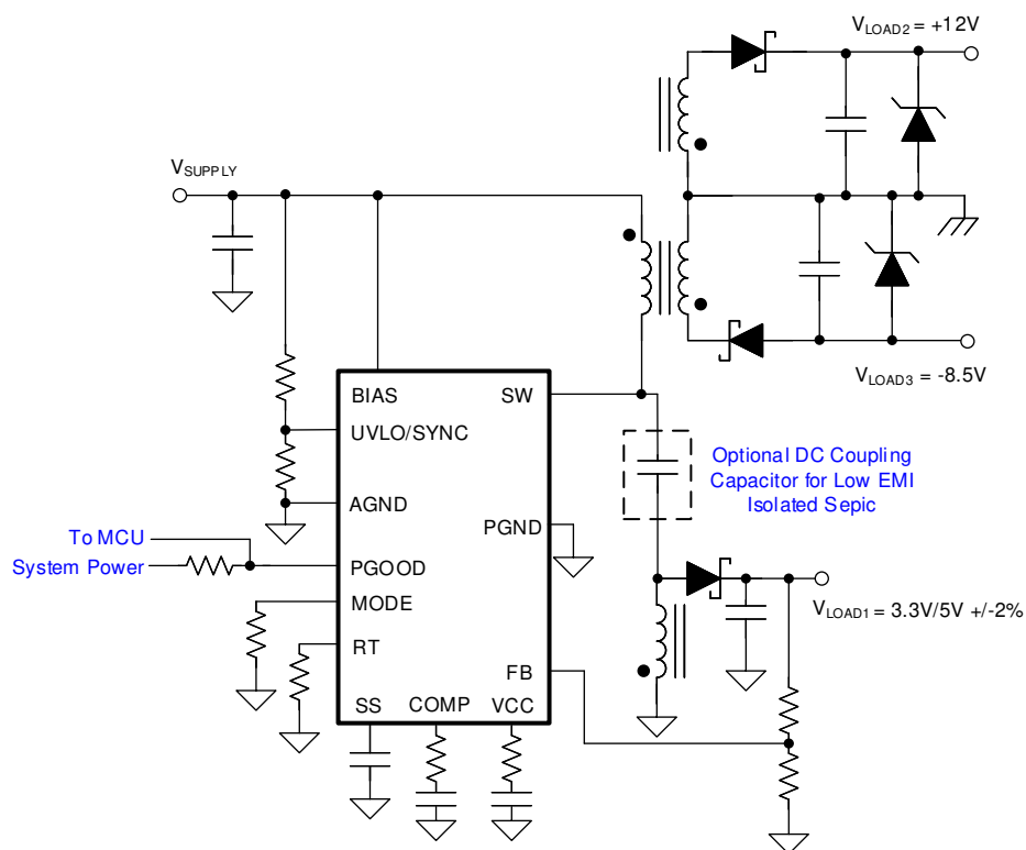
图 9-11. Primary-Side Regulated Multiple-Output Isolated Flyback/Isolated SEPIC
