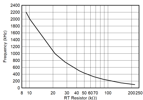
图 7-10. Frequency vs RT Resistance
