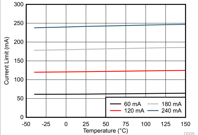
图 6-14. Peak Current Limits vs Temperature
