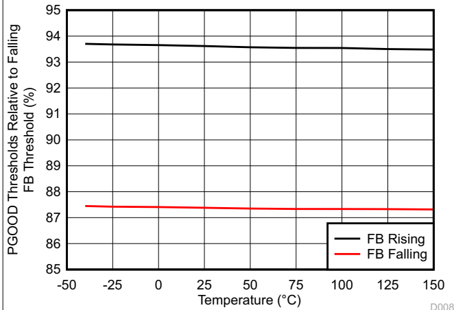
图 6-13. PGOOD Thresholds vs Temperature
