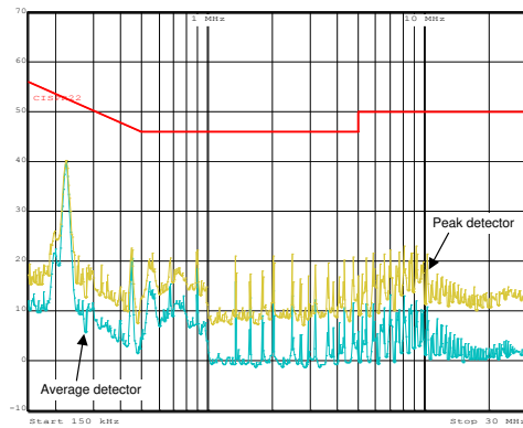
图 8-4. EMI Plot - CISPR 22 Filtered Emissions
