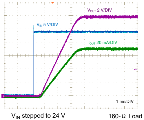
图 8-23. Start-Up, Full Load
