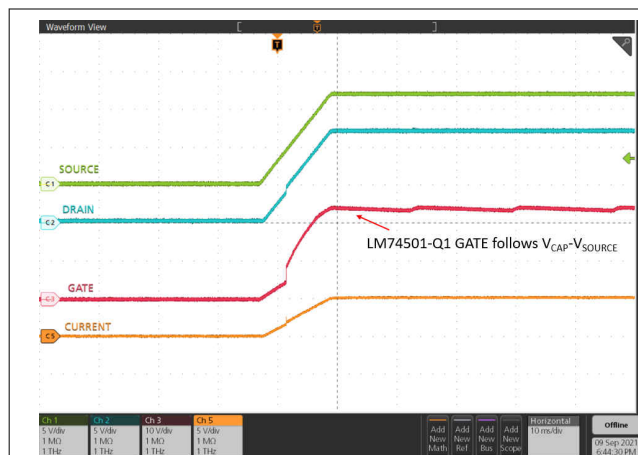
图 9-9. Start-up with 5-A Load
