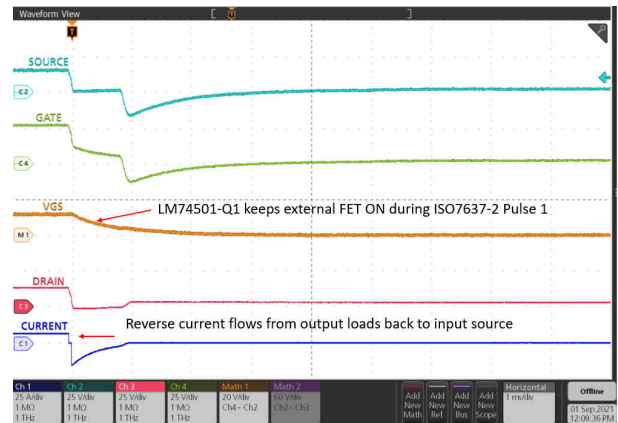
图 9-4. Response to ISO 7637-2 Pulse 1
