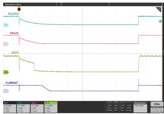
图 9-4. Response to ISO 7637-2 Pulse 1
