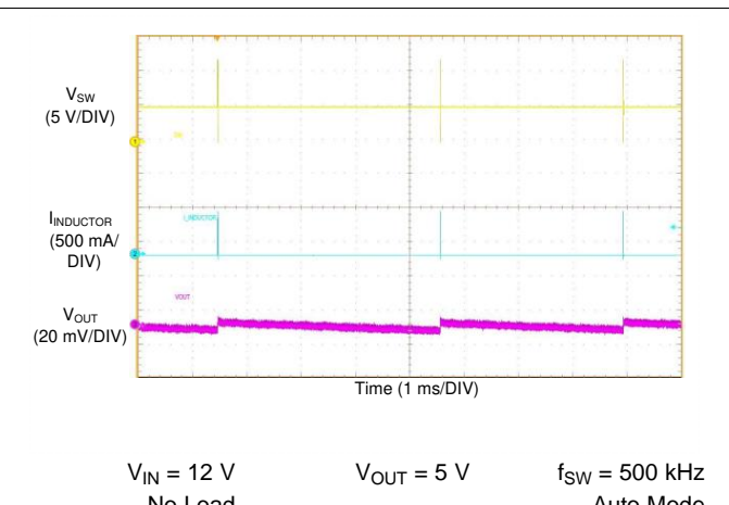
图 58. LM76003-Q1 Switching Waveform and Output Ripple
