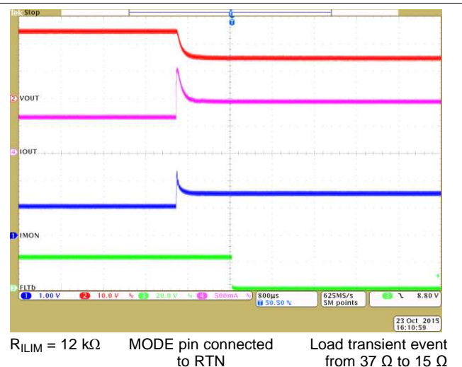
图 39. Output Turnoff Due to Thermal Shutdown With \overline{\text{FLT}} Asserted in Advance
