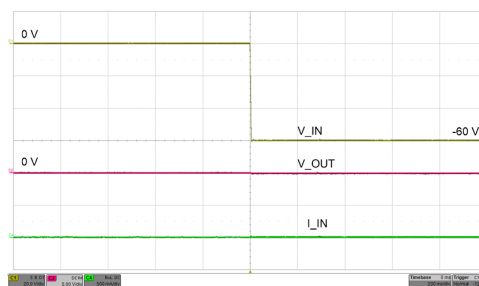
图 28. Reverse Input Supply Protection at -60 V
