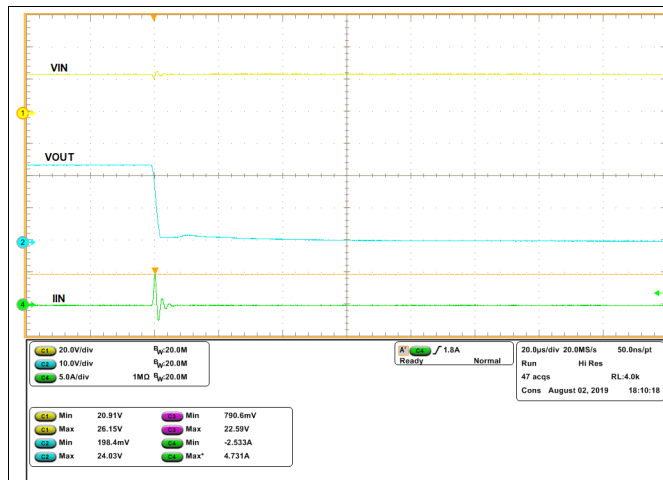
图 42. Protection from Output Short to GND [ V_{IN} = 24\text{ V} , I_{LIM} = 2.23\text{ A} , MODE = RTN ]
