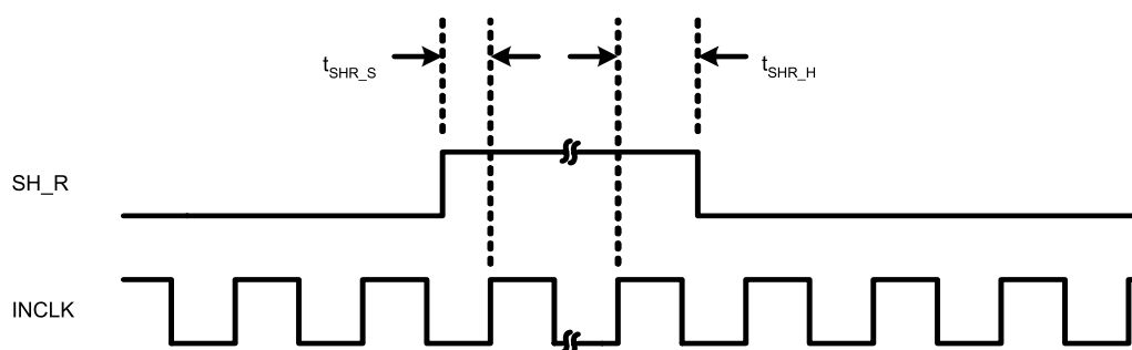
Figure 41. SH_R to INCLK (PIXCLK or ADCCLK) Timing
