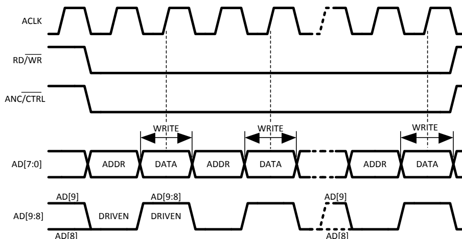
Figure 3. Control Data Write Timing
