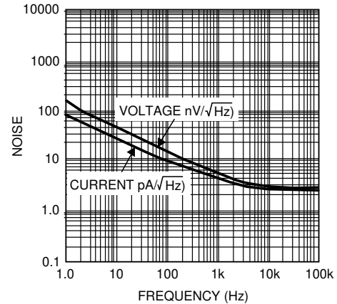
图 5-20. Noise vs. Frequency
