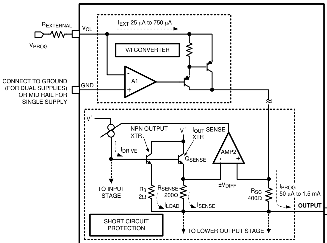
图 6-3. Simplified Diagram of Current Limit Control
