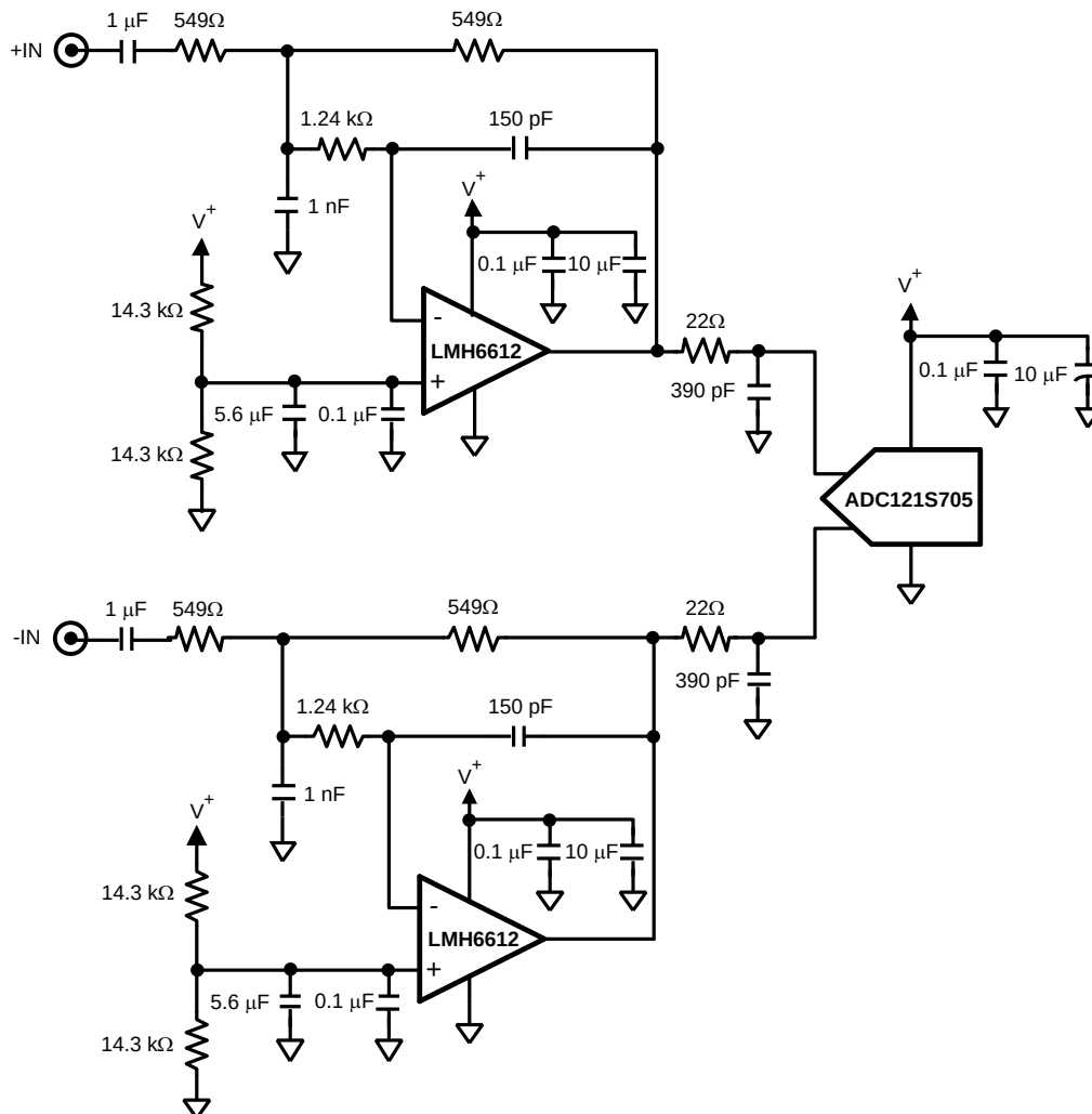
Figure 72. Differential to Differential ADC Driver
