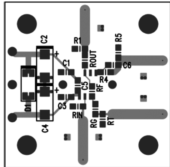
Figure 60. LMH6642/LMH6643/LMH6644 Layer 2
