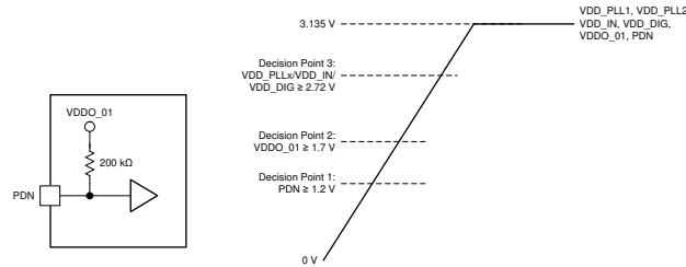
图 10-10. Recommendations for Power Up From Single-Supply Rail
