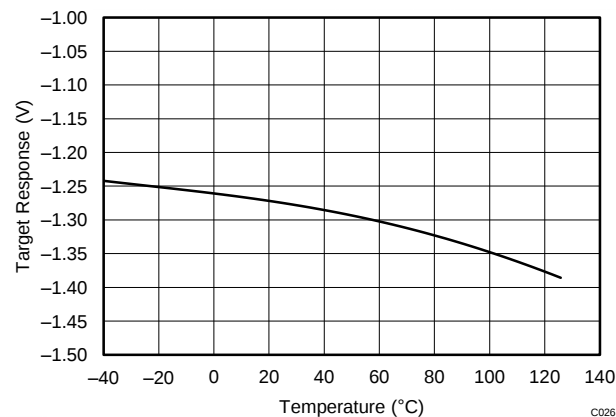
Figure 45. The Target Function to be Reproduced by the LMP92066: V_{GS} vs T Characteristic of a GaN PA
