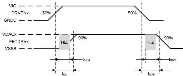
Figure 2. Switching
