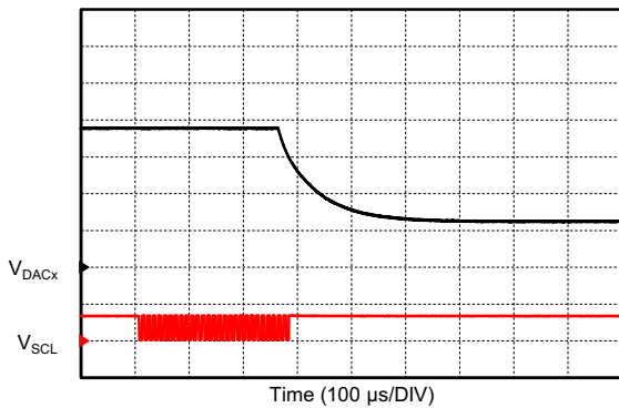
DAC OVERRIDE MODE C_L = 10\text{ }\mu\text{F} I^2\text{C} command triggers DAC step Step size: 3/4 to 1/4 FS
