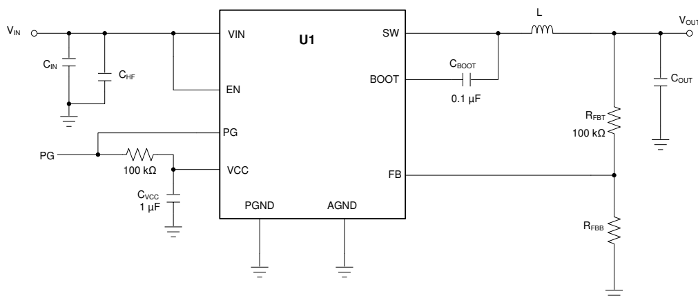
图 9-31. Circuit for Application Curves
