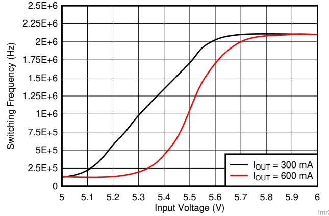
图 17. Typical f_{SW} vs Output Current f_{SW} = 2100\text{ kHz}
