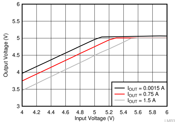
图 9-9. Overall Dropout Characteristic V OUT = 5 V
