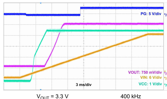
图 10-15. Start-Up Waveform
