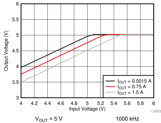
图 10-30. Overall Dropout Characteristic
