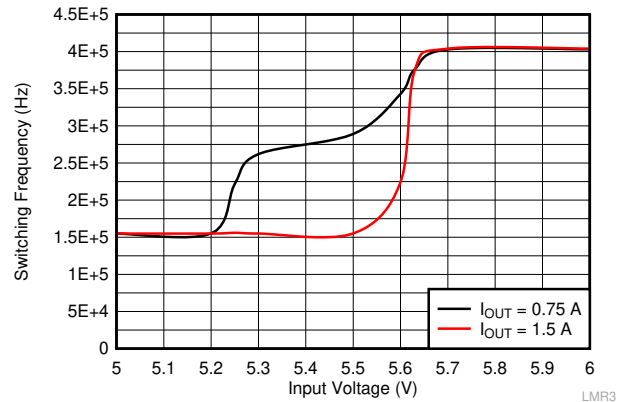
图 9-10. Frequency Dropout Characteristics f_{sw} = 400 \text{ kHz}
