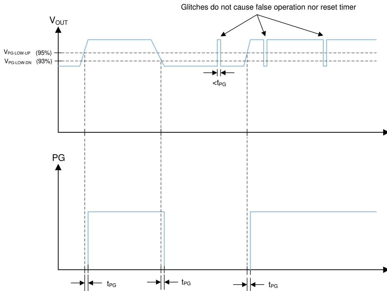
图 9-3. Power-Good-Timing Behavior
