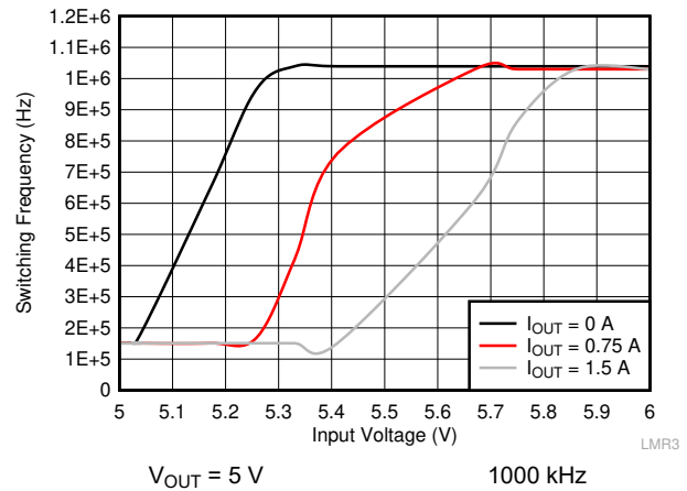
图 10-31. Frequency Dropout Characteristic
