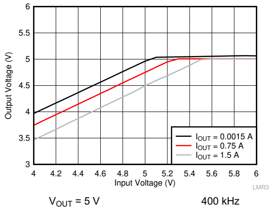
图 10-10. Overall Dropout Characteristic
