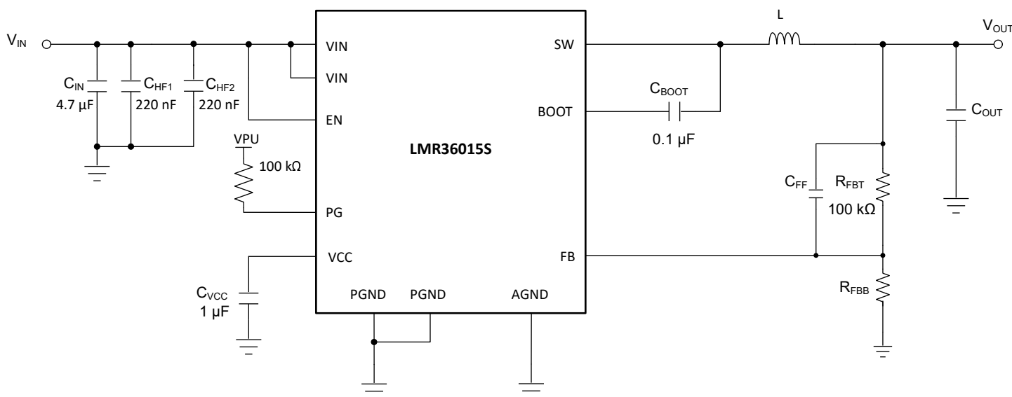
图 10-1. Example Applications Circuit
