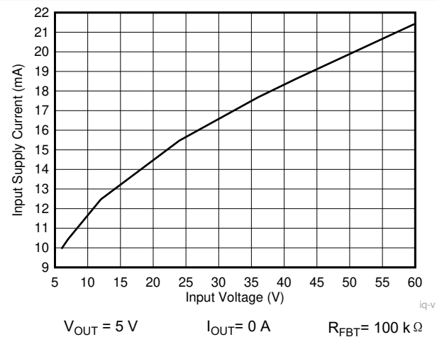
图 10-32. Input Supply Current
