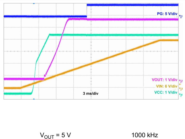
图 10-33. Start-Up Waveform
