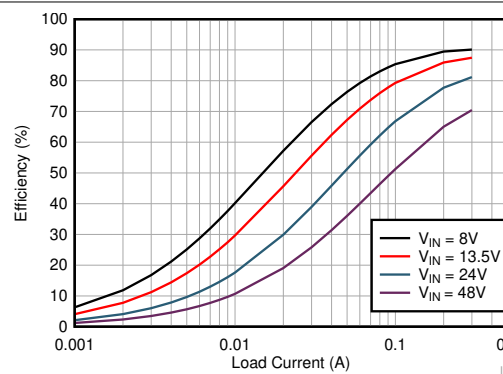
LMR36503MSC5 V_{OUT} = 5 V Fixed 2.2 MHz (FPWM)
