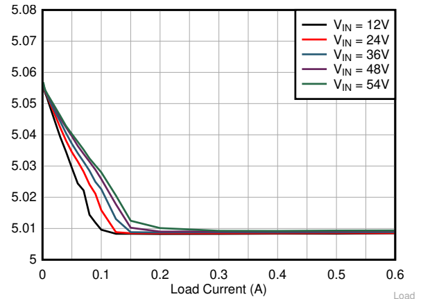
LMR36506R5 V_{OUT} = 5V 1MHz (自动)
