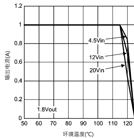
热降额V OUT = 1.8V
