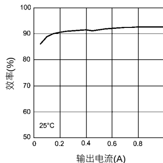
效率 V_{IN} = 12\text{V} V_{OUT} = 5.0\text{V}
