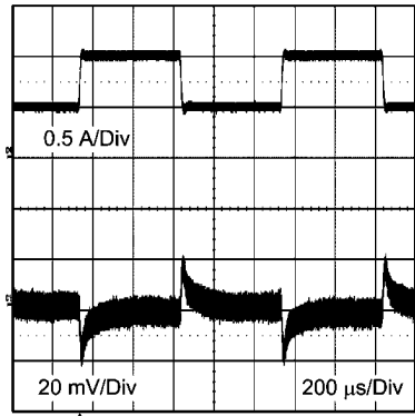
瞬态响应 12V IN 3.3V O 0.6A to 1A Step
