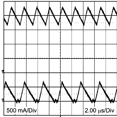
连续传导(CCM)与非连续传导运行模式 V_{IN} = 12V , V_O = 3.3V , I_O = 2A/0.26A 2 \mu sec/div
