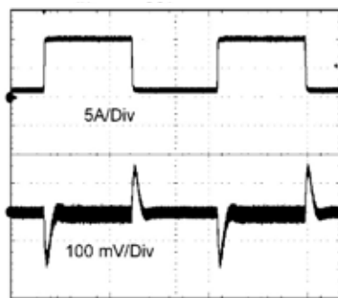
瞬态响应 12 V IN , 5.0 V OUT (1 A 至 10 A 阶跃)
