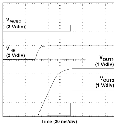
Figure 36. Sequencing Waveforms
