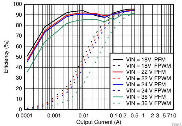
图 9-24. Efficiency
