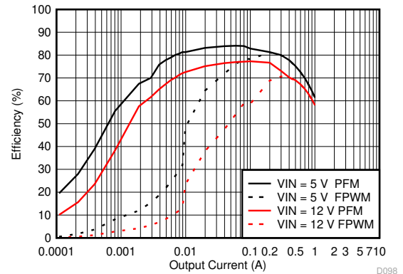
图 8-37. Efficiency for V_{OUT} = 1.2\text{ V}
