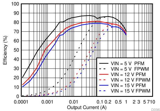
图 8-36. Efficiency for V_{OUT} = 1.8\text{ V}
