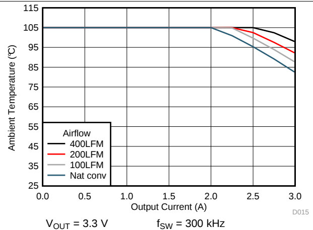
图 15. Safe Operating Area
