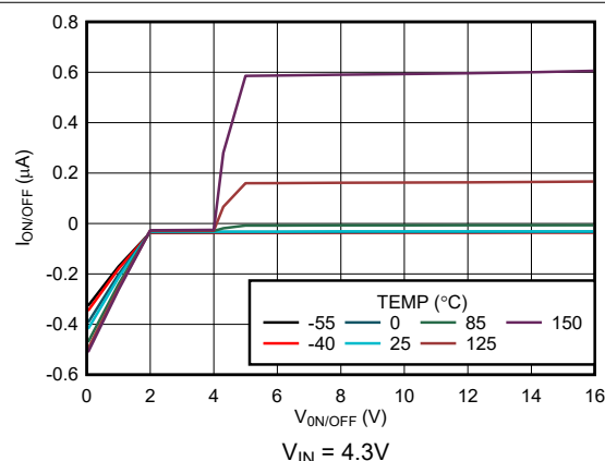
图 5-40. ON/OFF Pin Current vs V_{ON/OFF} (New Chip)
