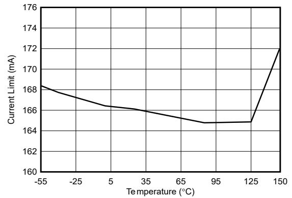
图 5-20. Short-Circuit Current vs Temperature (New Chip)
