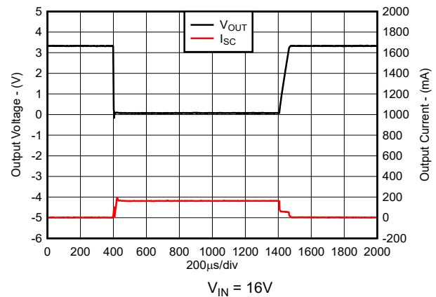
图 5-22. Short-Circuit Current vs Time (New Chip)
