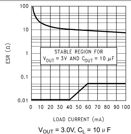
图 7-6. 3.0V, 10 \mu\text{F} ESR Curves (Legacy Chip)
