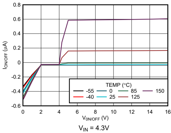
图 5-55. \overline{\text{ON/OFF}} Pin Current vs V_{\text{ON/OFF}} (New Chip)
