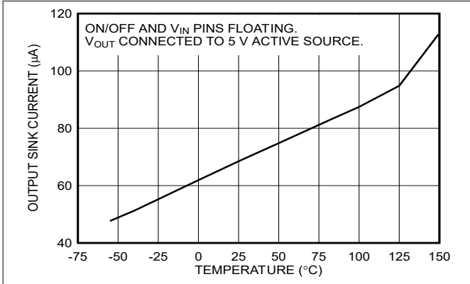
图 5-49. Output Reverse Leakage vs Temperature (New Chip)
