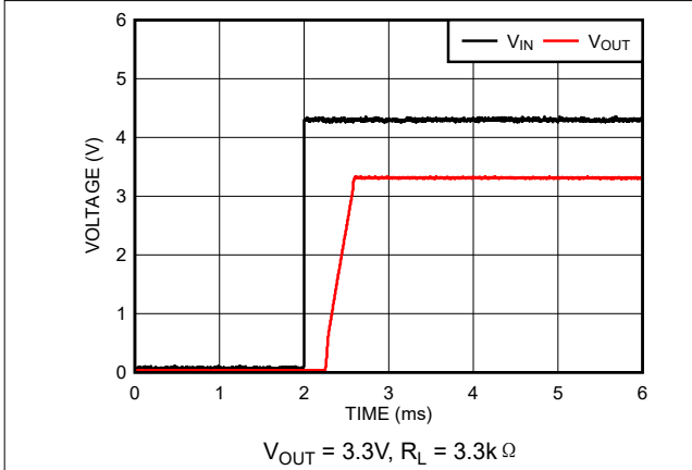
图 5-51. Turn-On Waveform (New Chip)
