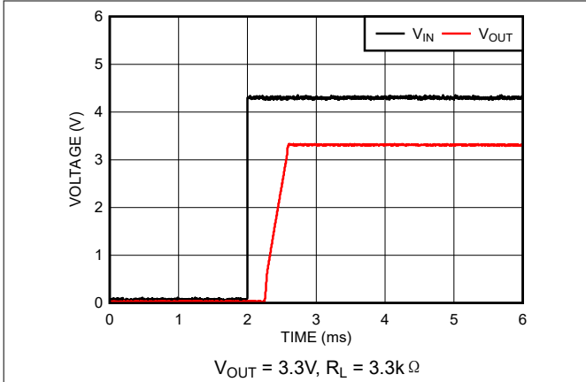
图 5-25. Turn-On Waveform (New Chip)
