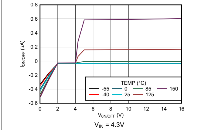
图 5-27. \text{ON}/\overline{\text{OFF}} Pin Current vs V_{\text{ON}/\overline{\text{OFF}}} (New Chip)
