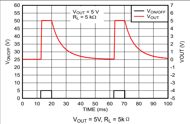
图 5-26. Turn-Off Waveform (New Chip)
