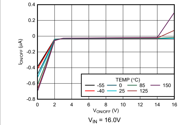
图 5-28. \text{ON}/\overline{\text{OFF}} Pin Current vs V_{\text{ON}/\overline{\text{OFF}}} (New Chip)
