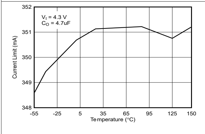
图 5-15. Short-Circuit Current vs Temperature for New Chip
