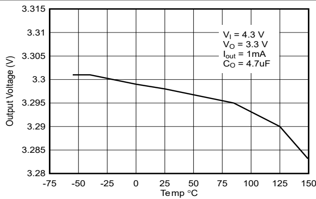
图 5-1. Output Voltage vs Temperature for Legacy Chip
