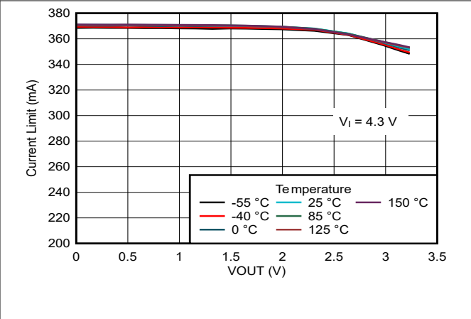
图 5-14. Short-Circuit Current vs Output Voltage for New Chip
