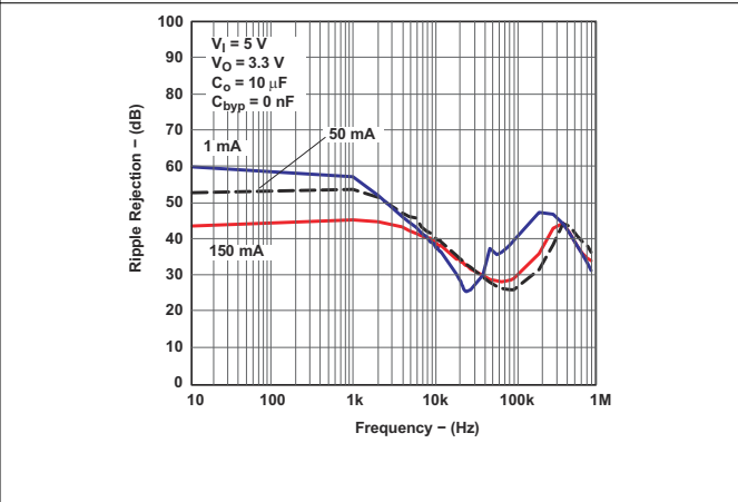
图 5-18. Ripple Rejection vs Frequency for Legacy Chip
