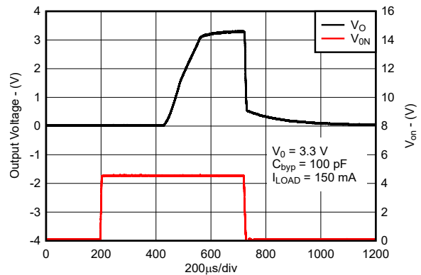
图 7-18. Turn-On Time for New Chip
