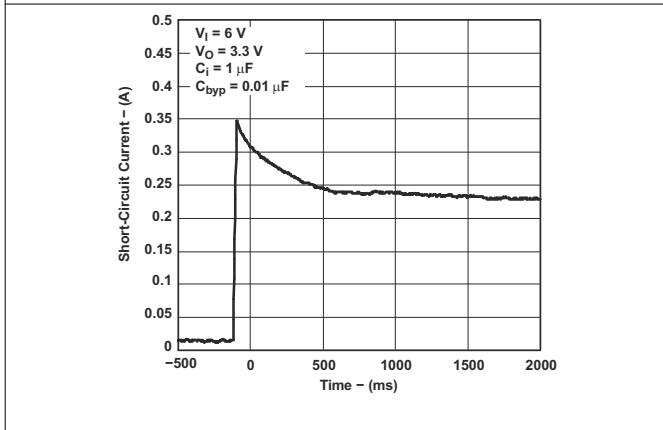
图 5-9. Short-Circuit Current vs Time for Legacy Chip
