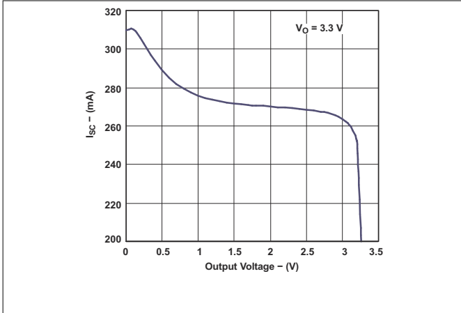
图 5-13. Short-Circuit Current vs Output Voltage for Legacy Chip
