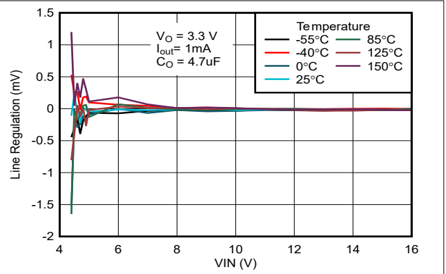
图 5-8. Output Regulation vs Input Voltage for New Chip
