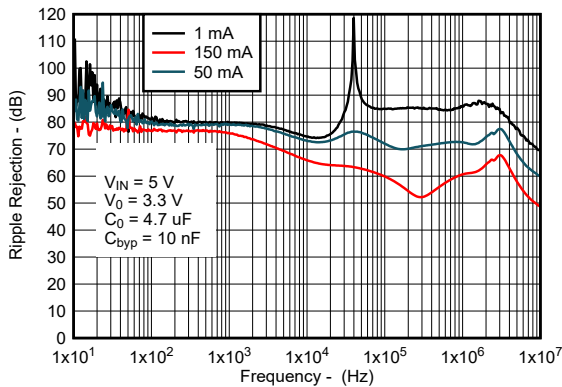
图 5-21. Ripple Rejection vs Frequency for New Chip
