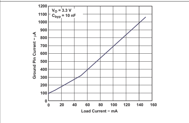
图 5-16. Ground Pin Current vs Load Current for Legacy Chip
