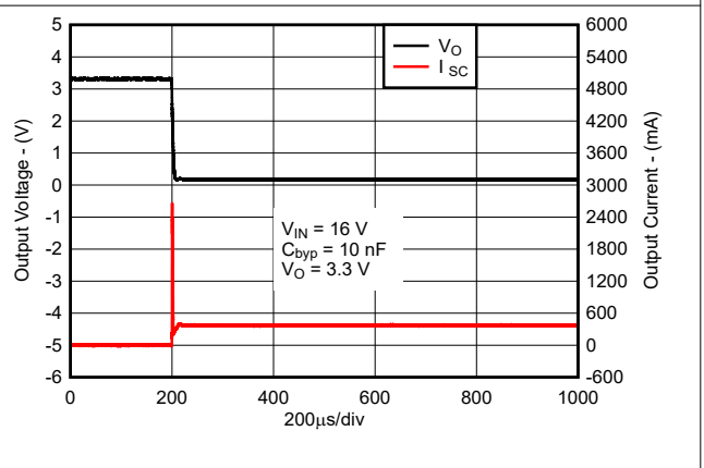
图 5-12. Short-Circuit Current vs Time for New Chip
