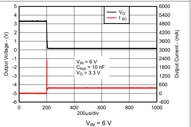
图 5-10. Short-Circuit Current vs Time for New Chip
