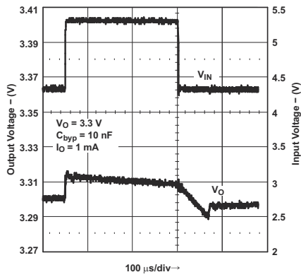
图 7-15. Line Transient Response for Legacy Chip
