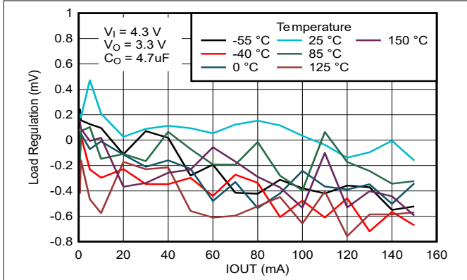
图 5-7. Output Regulation vs Load Current for New Chip
