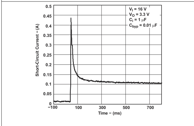
图 5-11. Short-Circuit Current vs Time for Legacy Chip
