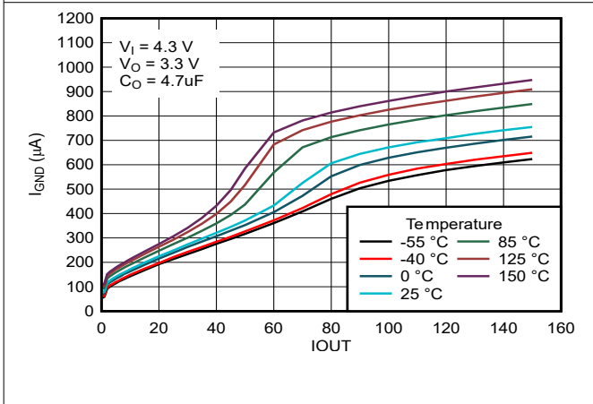
图 5-17. Ground Pin Current vs Load Current for New Chip
