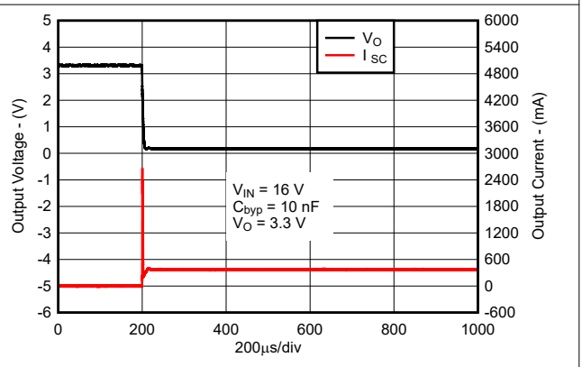
图 5-10. Short-Circuit Current vs Time for New Chip
