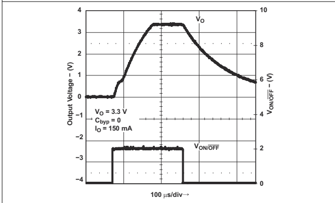
图 7-17. Turn-On Time for Legacy Chip
