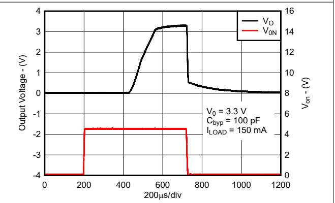
图 7-18. Turn-On Time for New Chip
