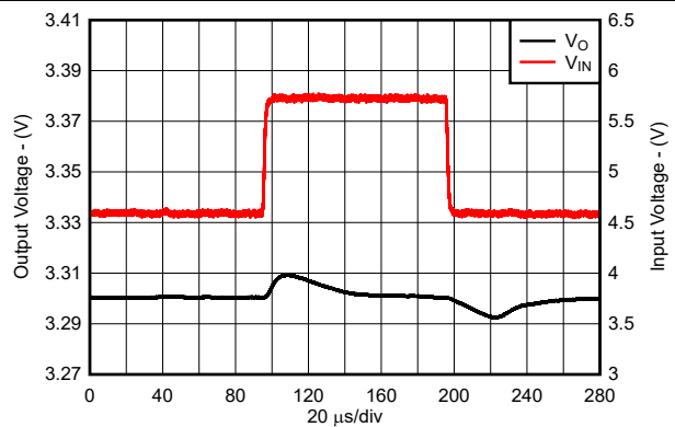
图 7-12. Line Transient Response for New Chip
