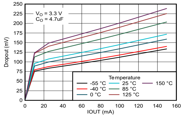
图 5-4. Dropout Voltage vs Temperature for Legacy Chip
