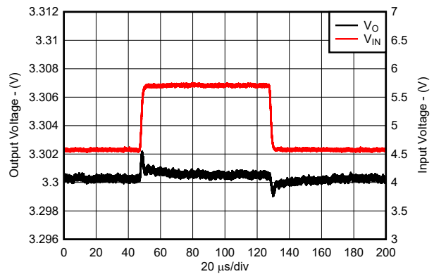
图 7-10. Line Transient Response for New Chip
