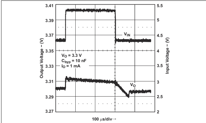
图 7-15. Line Transient Response for Legacy Chip
