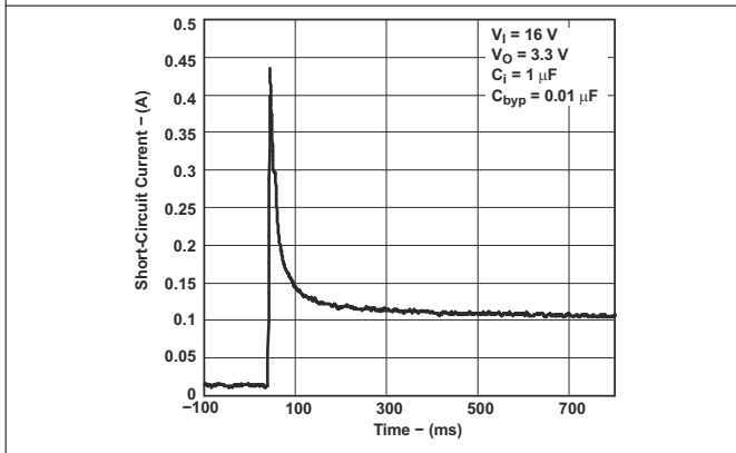
图 5-9. Short-Circuit Current vs Time for Legacy Chip
