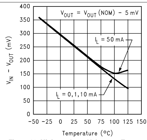
Figure 12. Minimum Input Voltage vs Temperature
