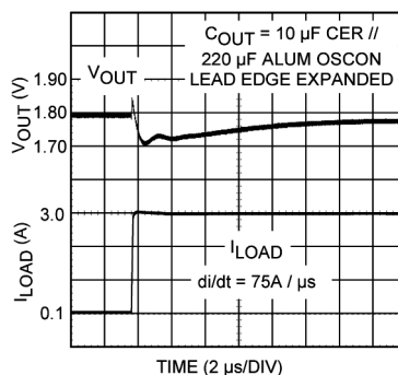
Figure 22. 10- \mu\text{F} Ceramic Paralleled by 220- \mu\text{F} OSCON
