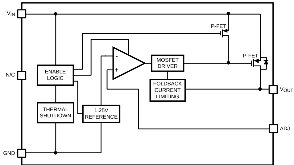
Figure 4. LP38690-ADJ Functional Diagram (WSON)
