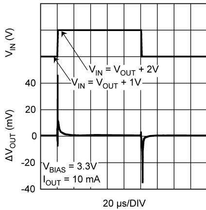
Figure 13. V_{IN} Line Transient Response
