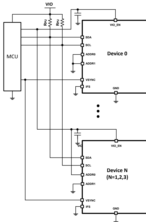
图 8-13. I²C Multiple Devices Connection
