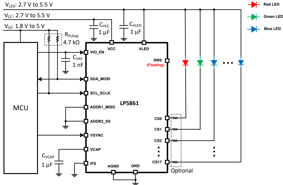
图 9-2. Typical Application 2 – LP5861 Drives Six RGB LEDs Without Internal Switch
