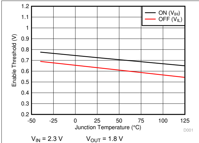
图 6-1. V_{EN} Threshold vs Temperature
