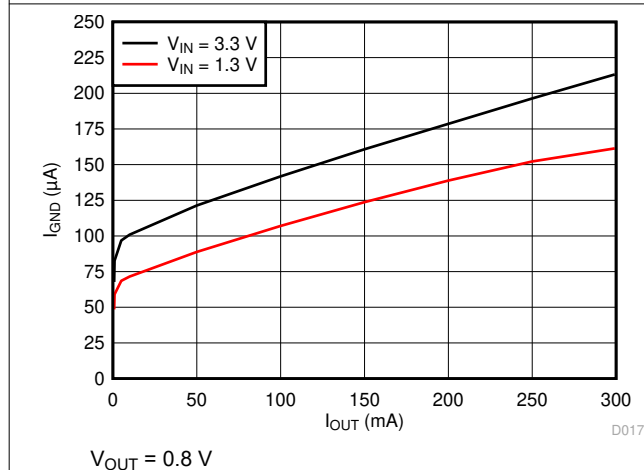
图 6-17. I_{GND} vs I_{OUT}
