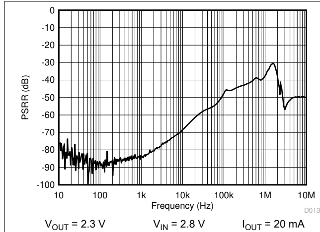
图 6-13. PSRR vs Frequency
