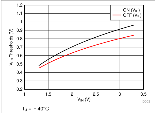
图 6-3. V_{EN} Thresholds vs V_{IN}
