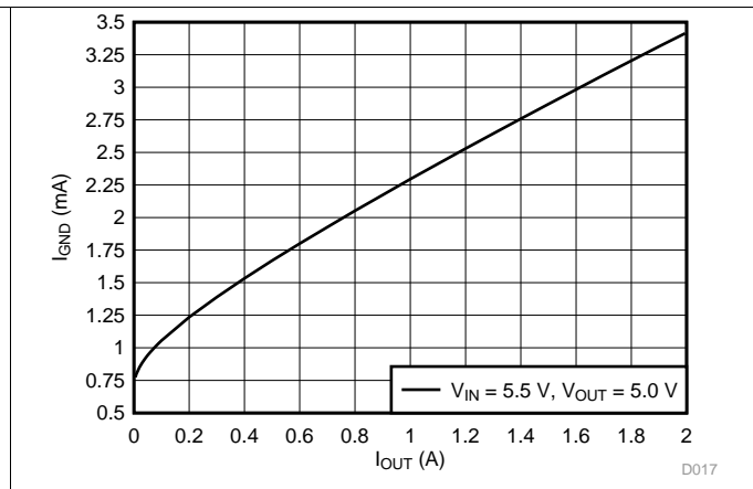
Figure 2. Ground Current vs Output Current
