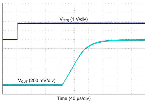
图 8-24. LDO Start-Up
