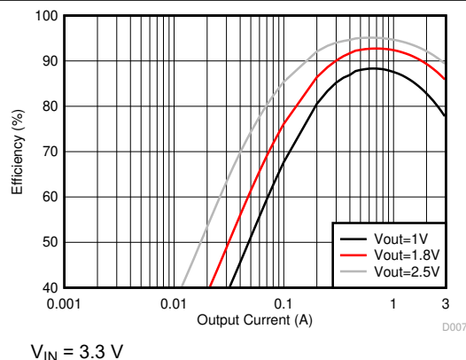
图 8-3. Buck Efficiency in Forced PWM Mode
