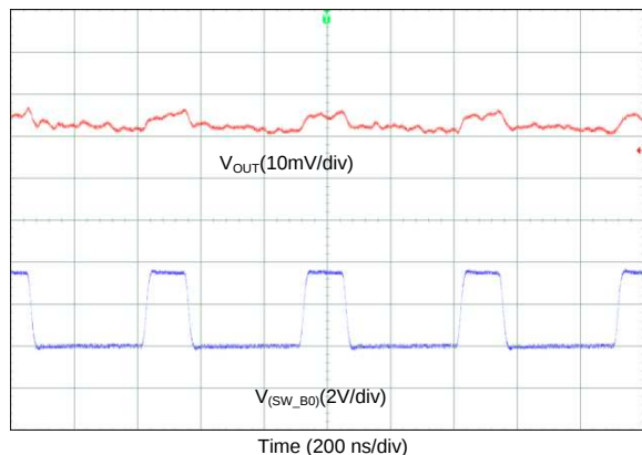
图 82. Output Voltage Ripple, Forced-PWM Mode (3-Phase Output)
